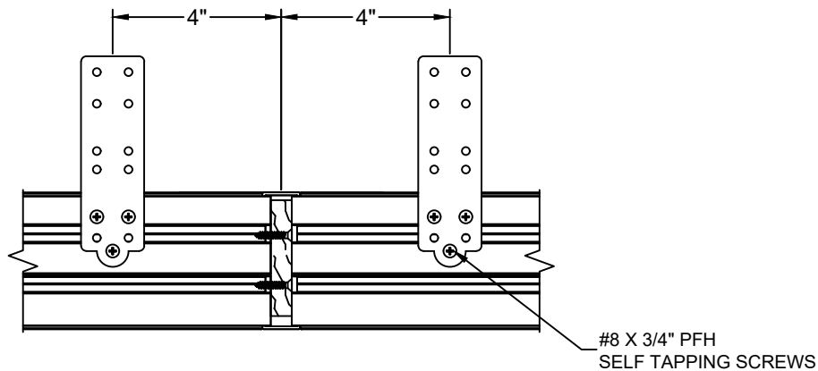
RED OAK REINFORCEMENT AT INSTALLATION STRAP DETAIL AT MULLS
